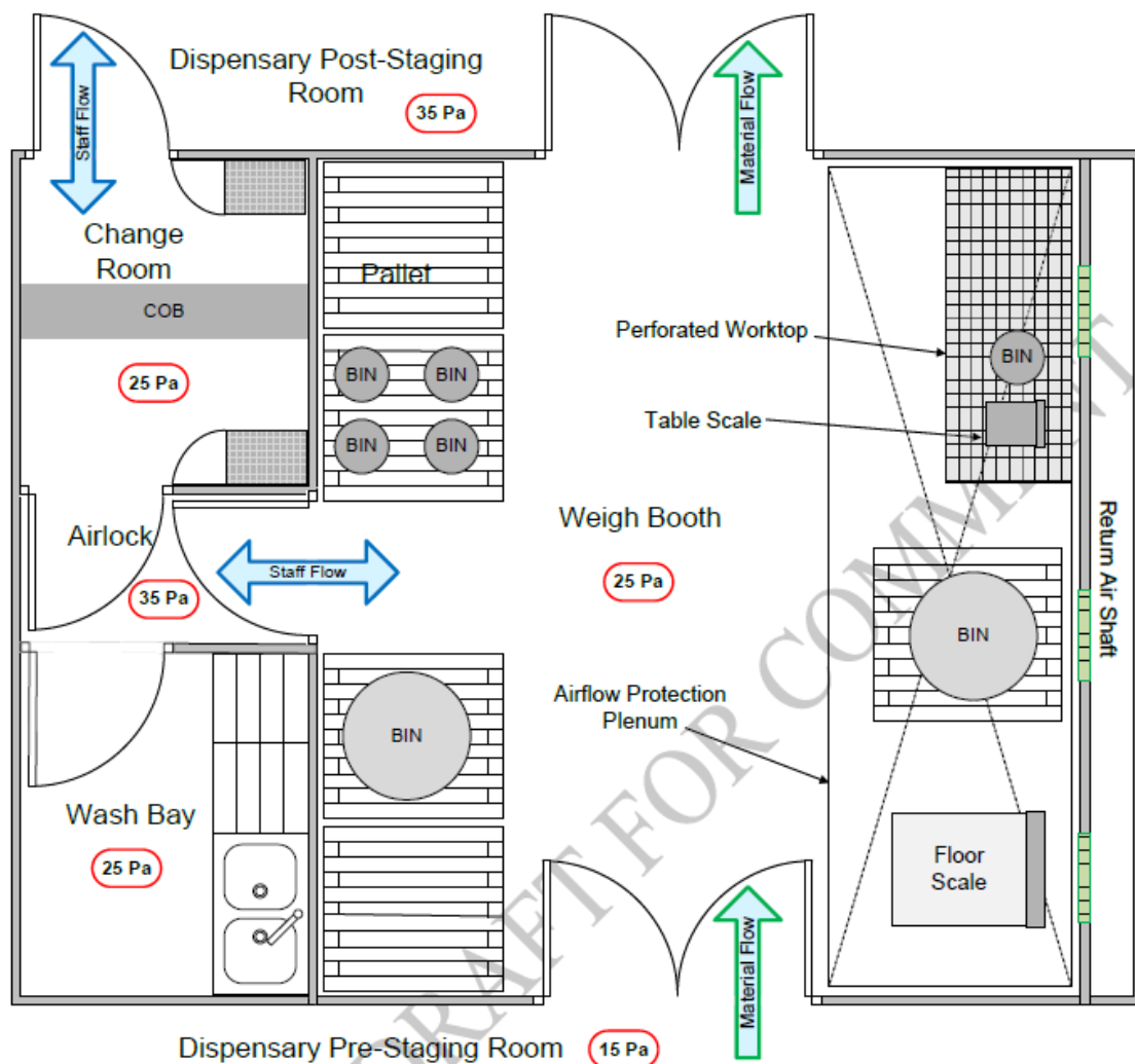
563 | Figure 3. Example of a weigh booth layout 564
